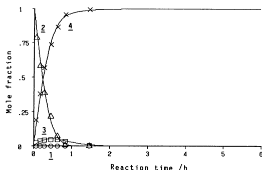
Fig. 6. Product distributions on the hydrogenation of 2 over Ru/Al 2 O 3 at 157°C under 100 atm H 2 pressure. See Fig. 2 for the chemical names of symbols.
